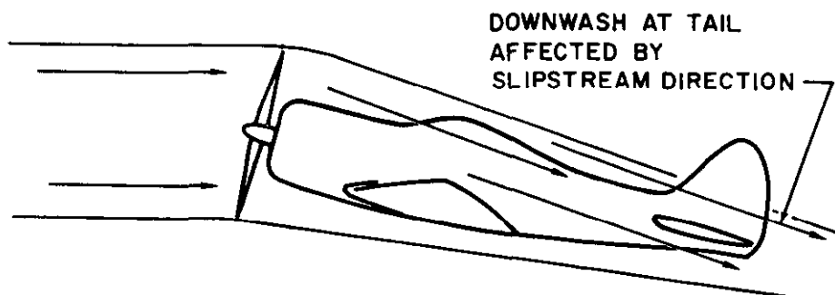
Figure 4.12. Indirect Power Effects.
