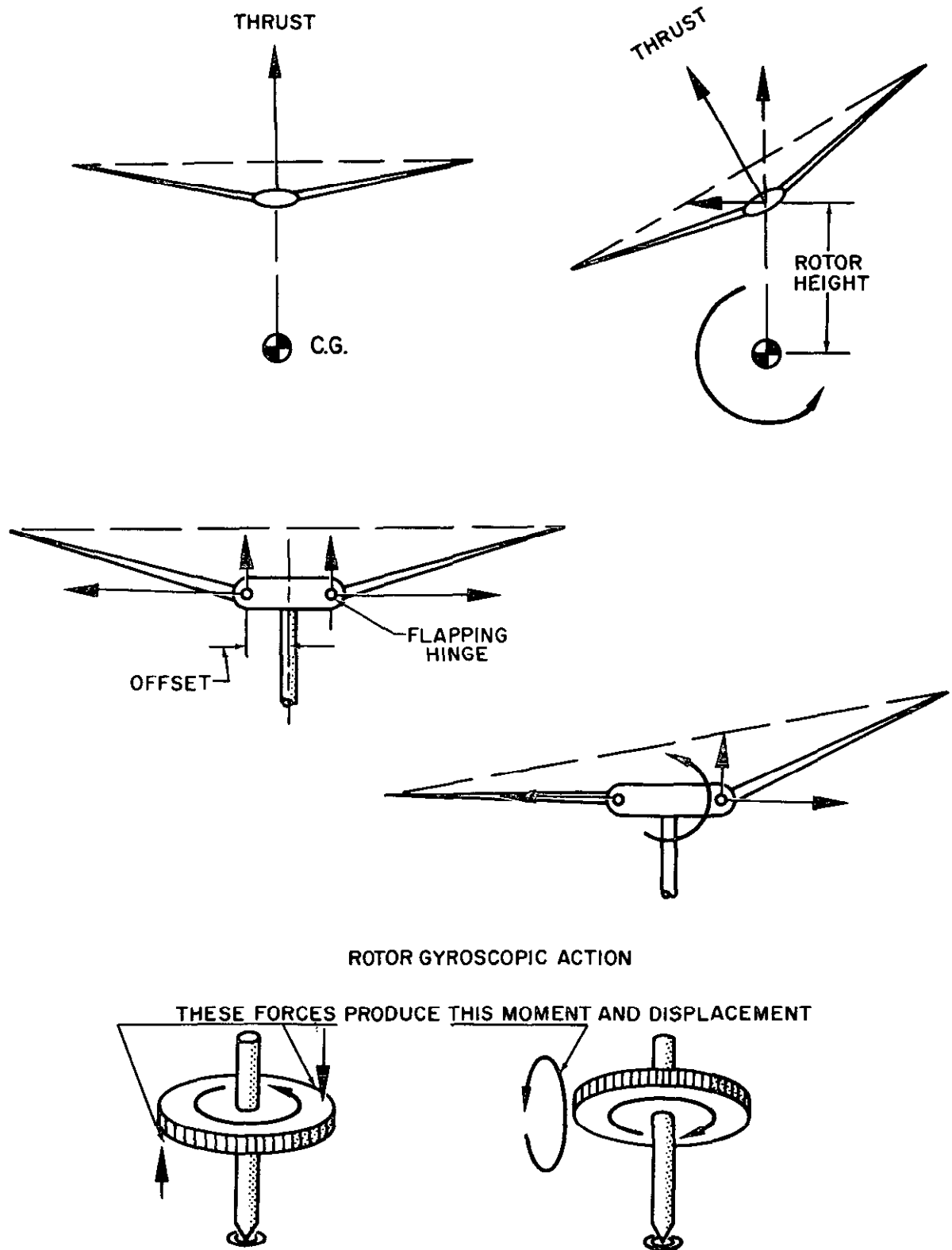
Figure 4.35. Rotor Forces and Moments
