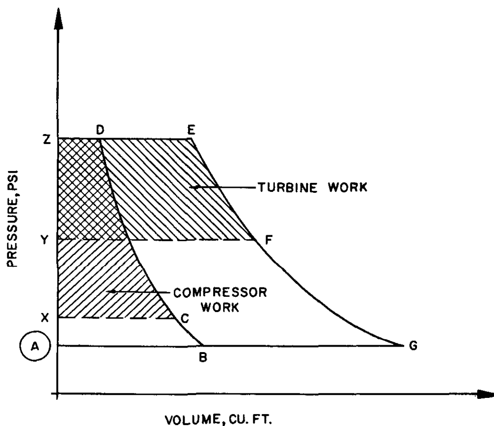
Figure 2.6. Turbojet Engines
