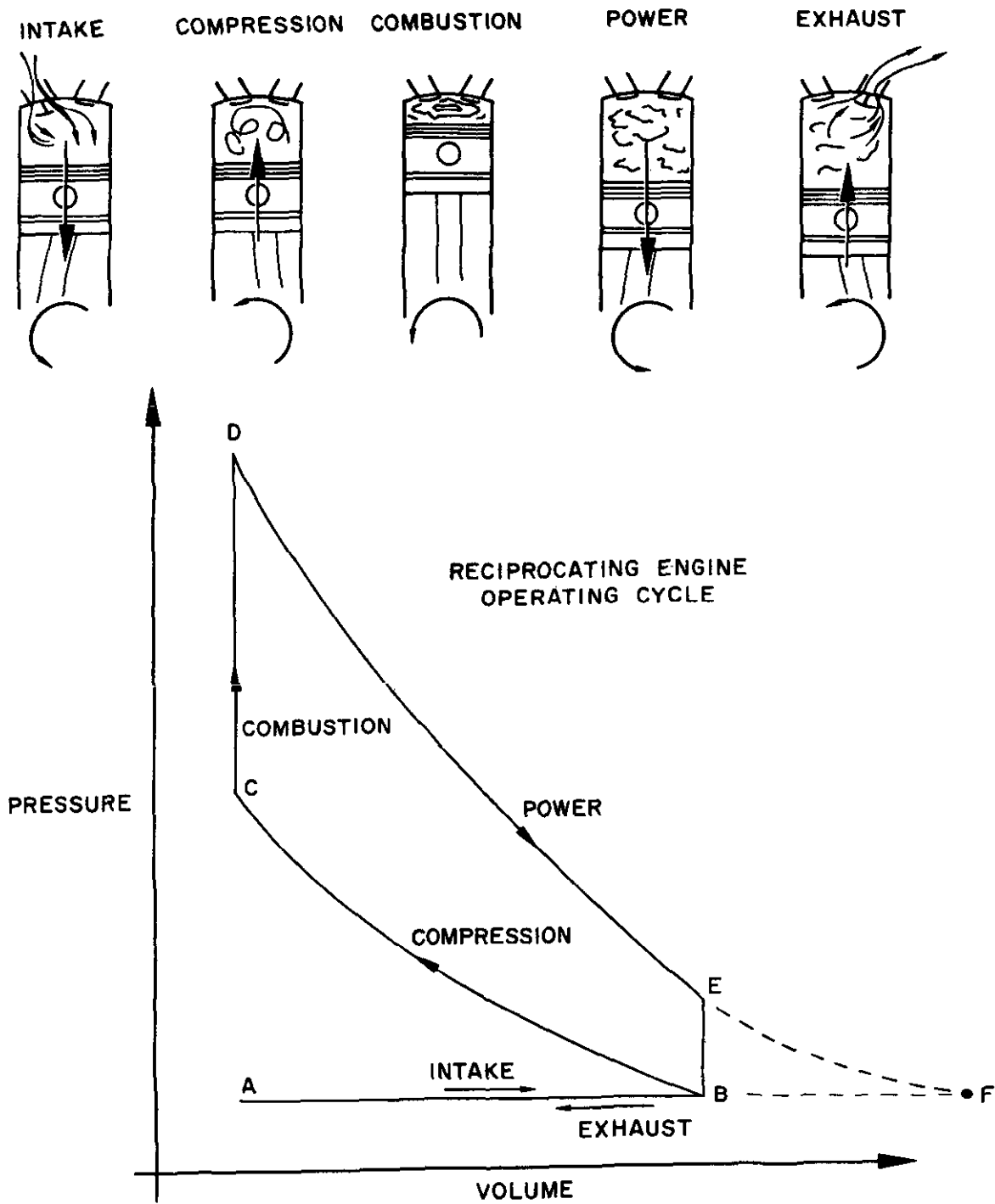
Figure 2.15. Reciprocating Engines
