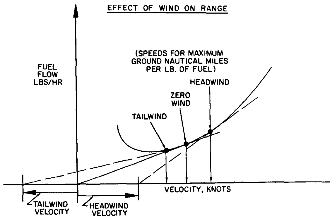
Figure 2.26. Range Performance
