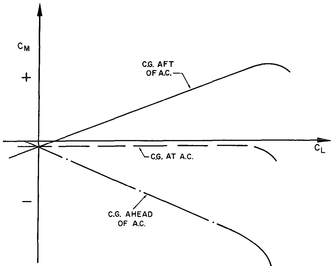
Figure 4.6. Wing Contribution
