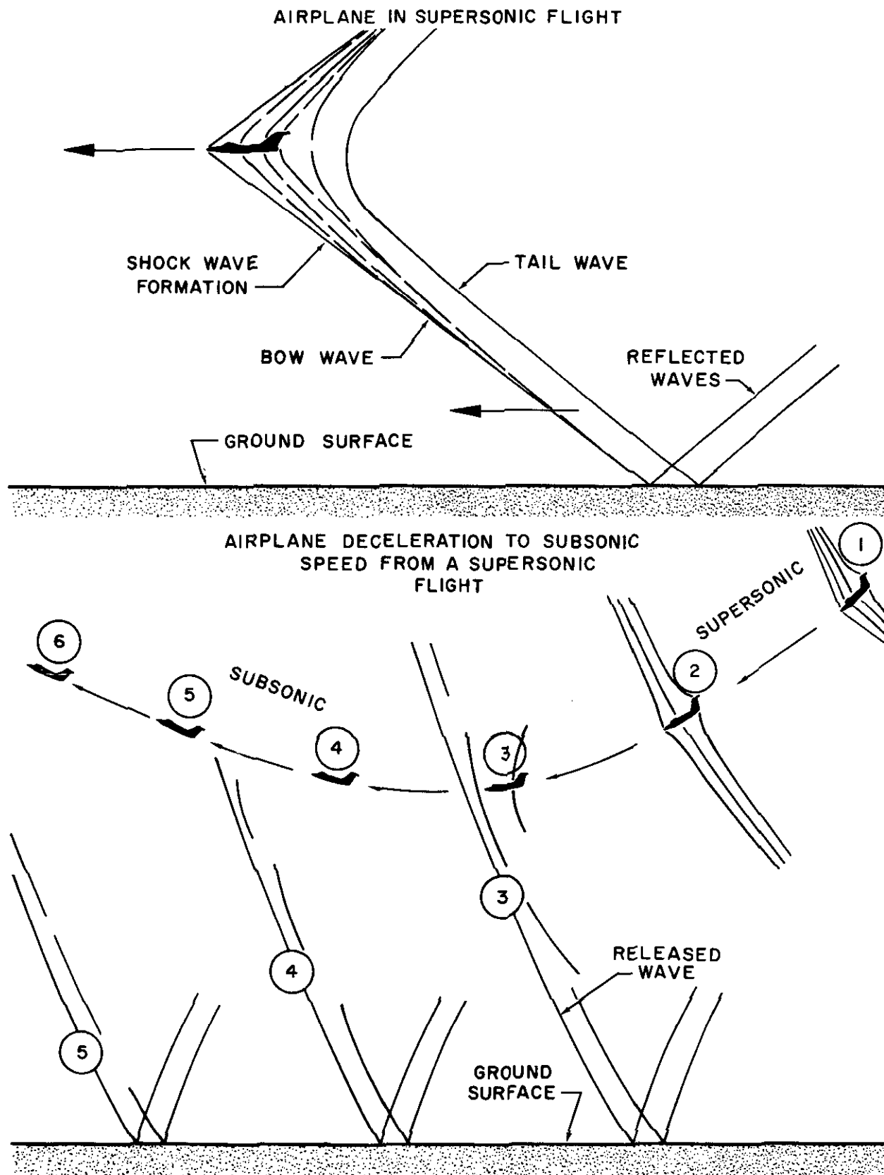
Figure 6.14. Sonic Booms
