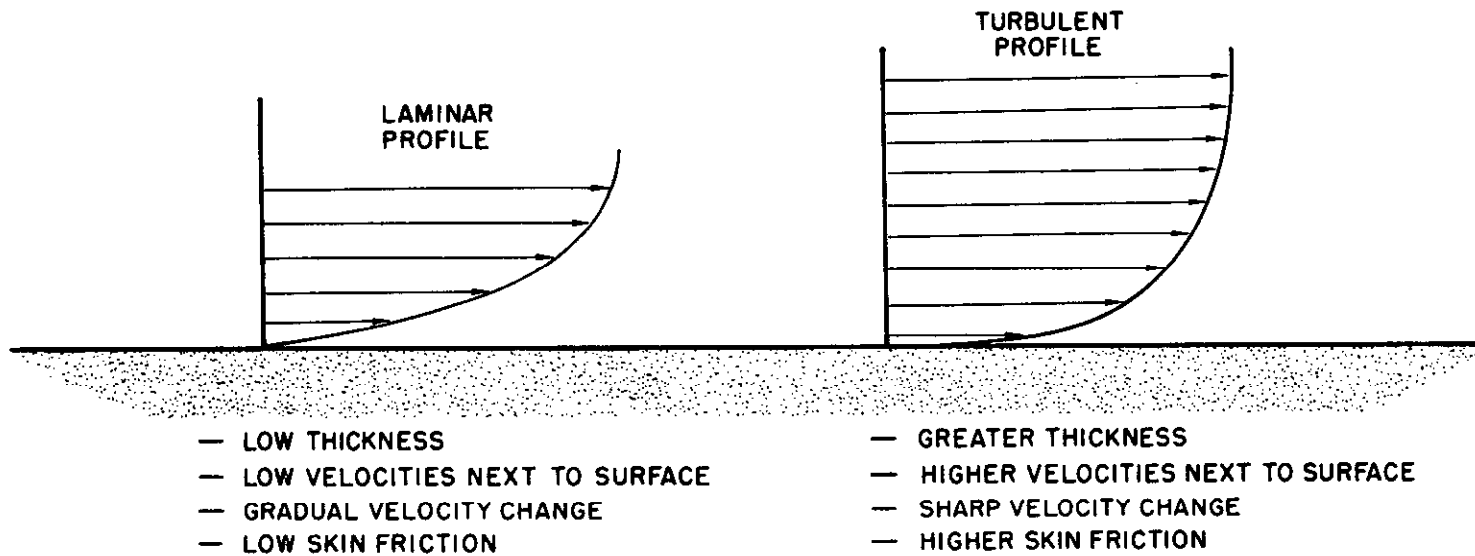
Figure 1.24. Boundary Layer Characteristics
